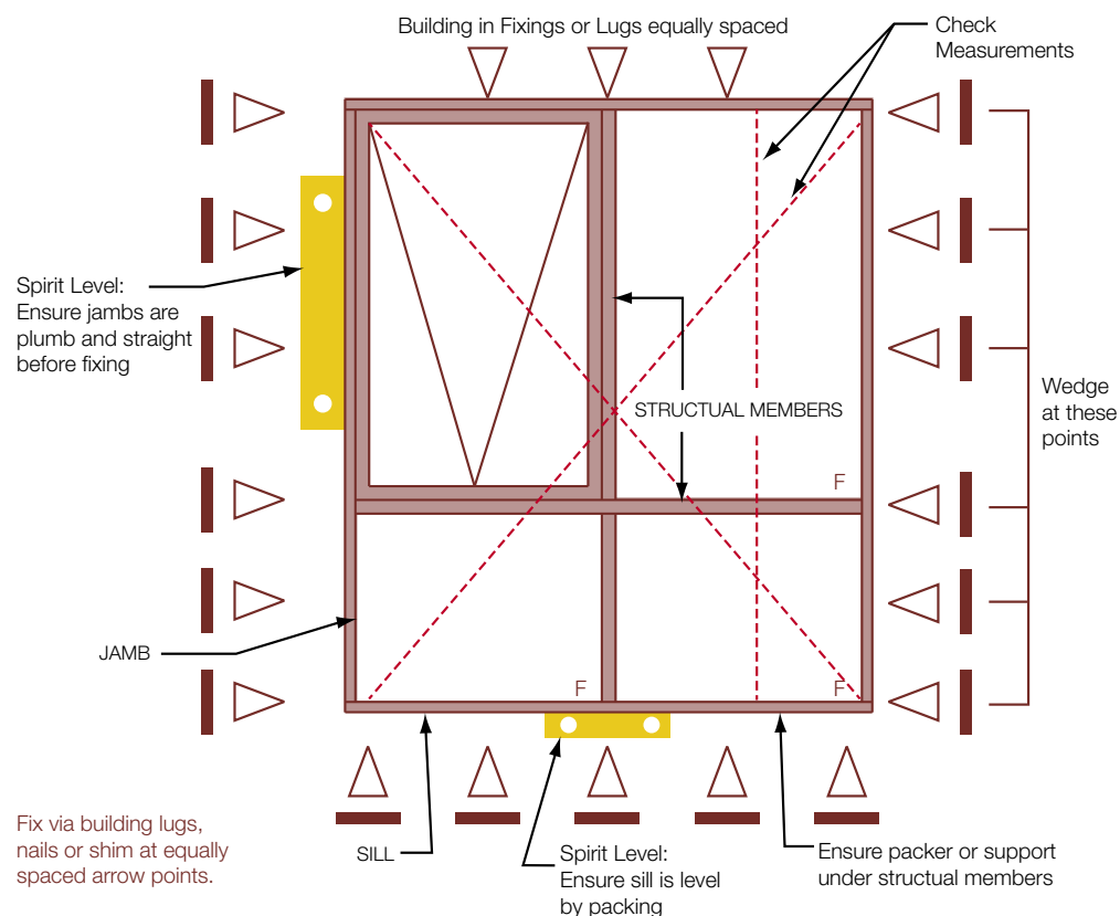
Figure 11 Installation Summary
